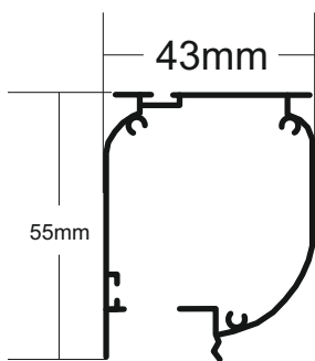
Contract Cassette Headbox
