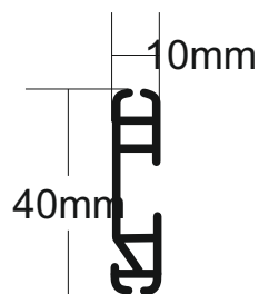
Contract Cassette Bottom Rail
