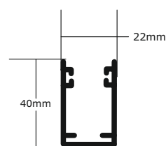
Side Channel
