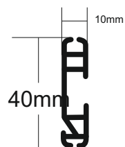
Contract Cassette Bottom Rail
