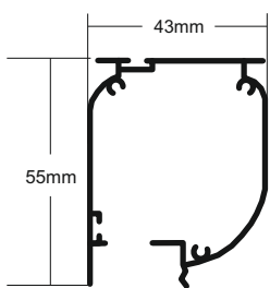
Contract Cassette Headbox
