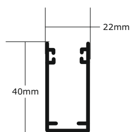
Side Channel
